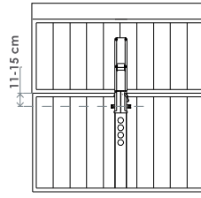
Folding door
